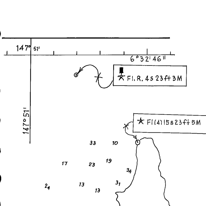
PLAN: LANGEMAK BAY AND FINSCH HARBOUR
