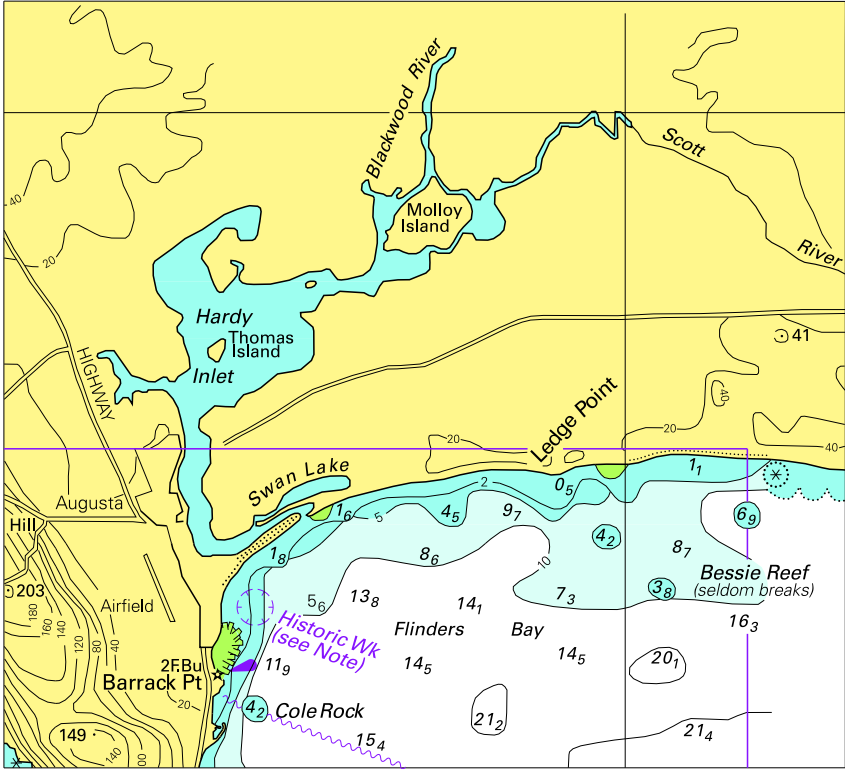
Block for Chart Aus 756 (111.3 x 101.4mm) © Commonwealth of Australia 2014
